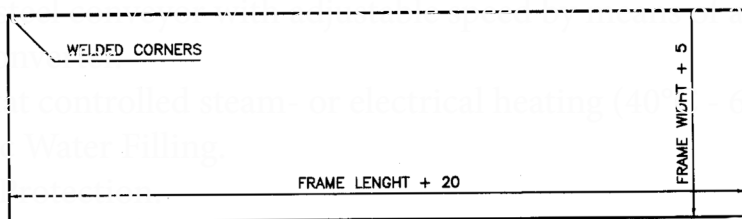
STANDARD DOUBLE TRAY BOTTOM 1,0 mm
