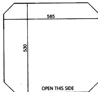
STANDARD DOUBLE LOOSE BOTTOM 1,0 mm
