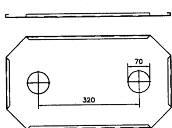
FIXED BOTTOM 0.8 MM
