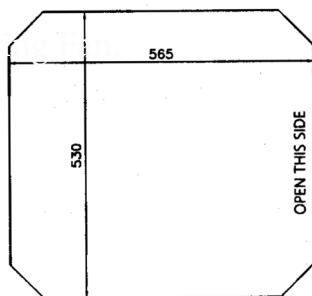
NORWEGIAN DOUBLE LOOSE BOTTOM
