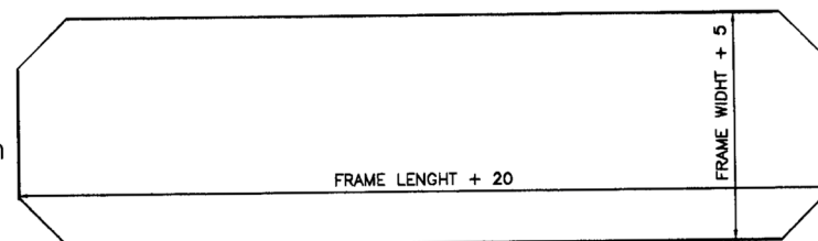
STANDARD DOUBLE LOOSE BOTTOM 1,0 mm
